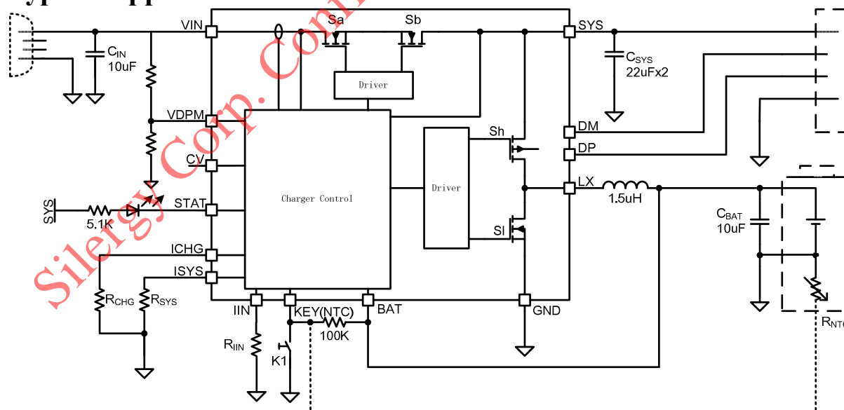
Figure 1. Schematic Diagram
