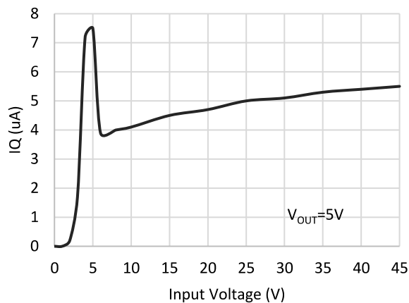
IQ vs. Input Voltage
